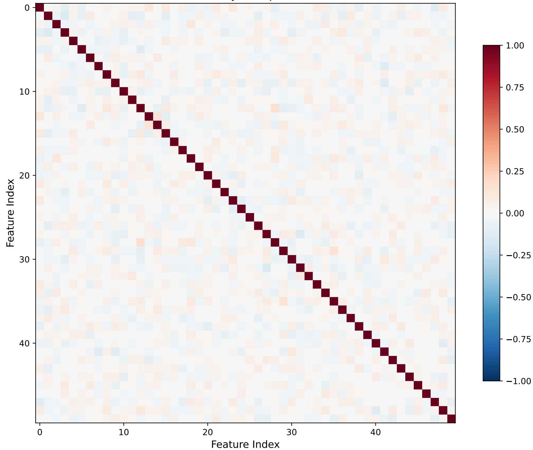
Pairwise Cosine Similarity of Top-50 Decoder Columns
