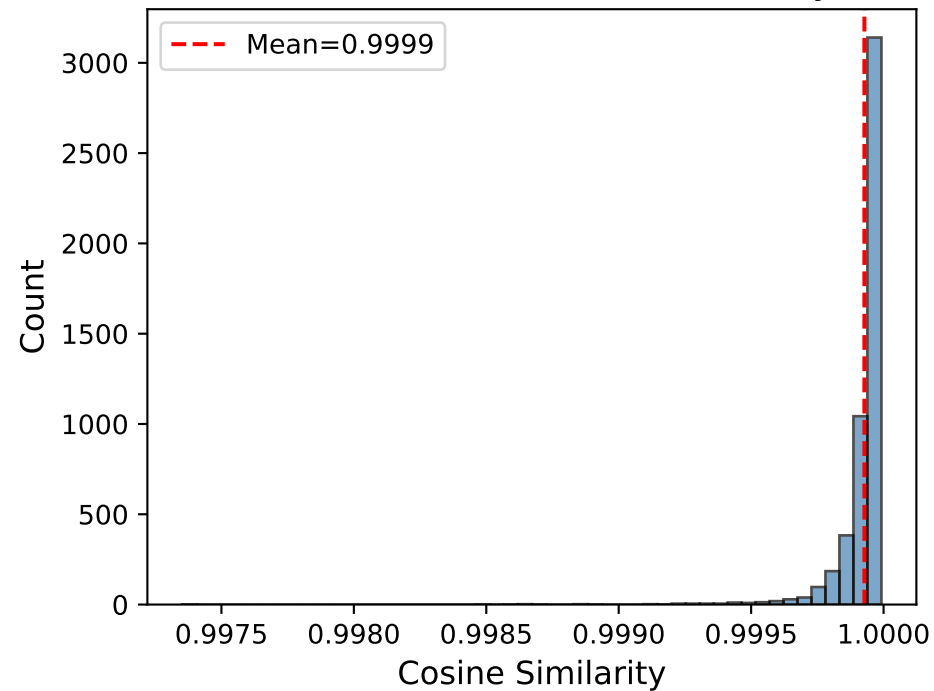
Reconstruction Cosine Similarity
