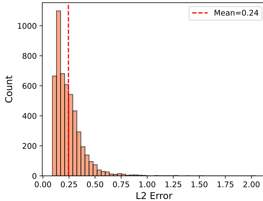
Reconstruction Error
