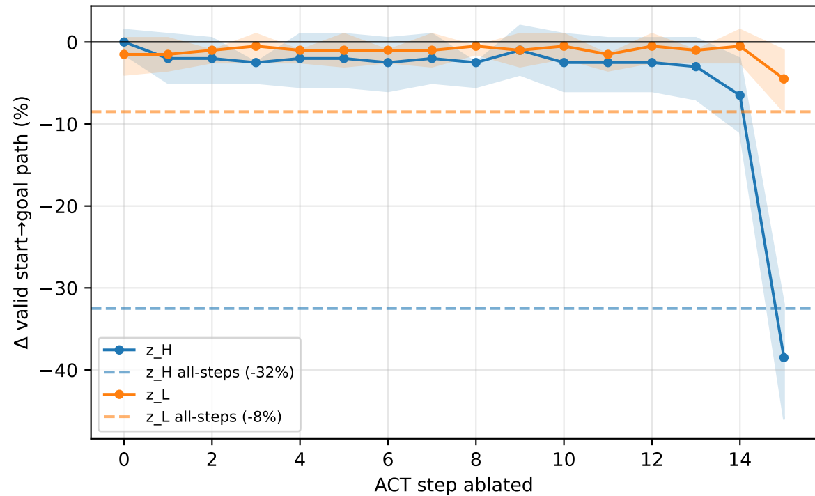
Maze — single-step ablation sensitivity (path-validity)
