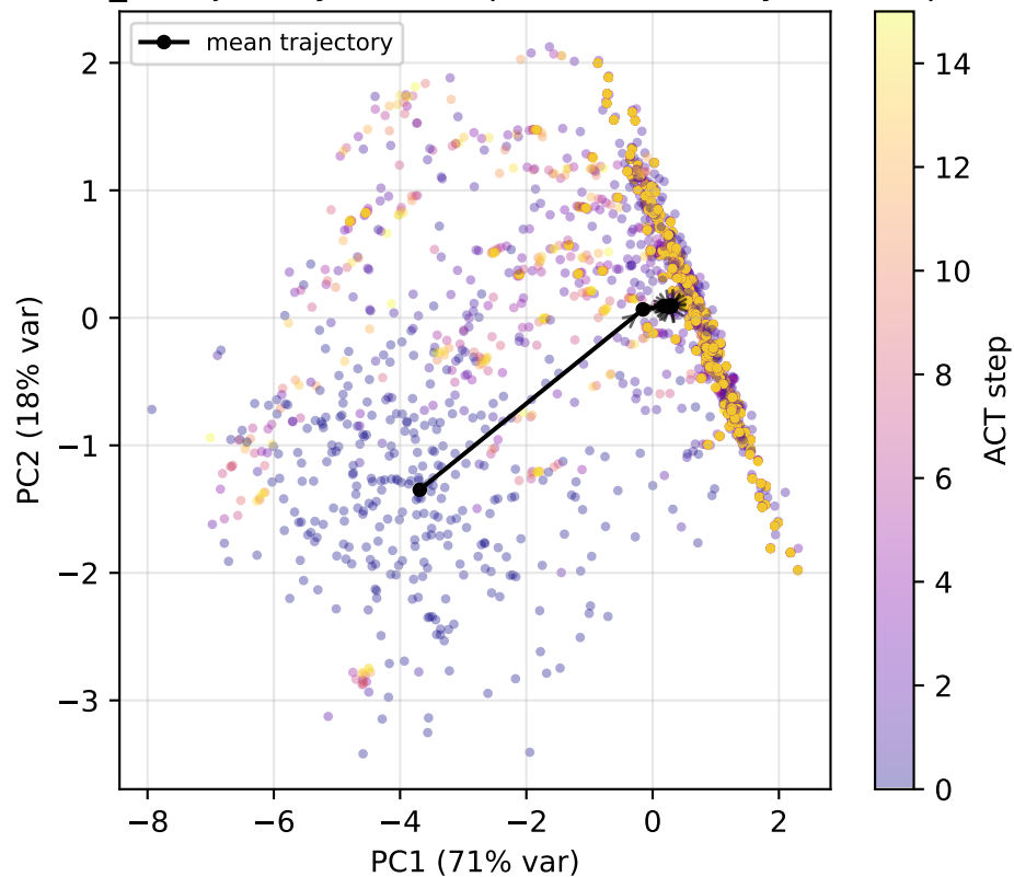
Maze z_H trajectory in PCA space (colored by ACT step)
