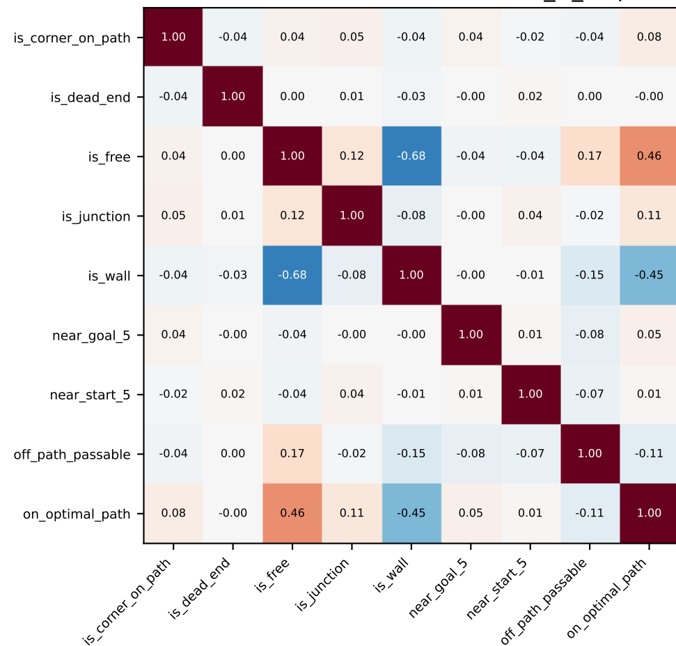
Feature-direction cosine matrix (z_H_step8)
