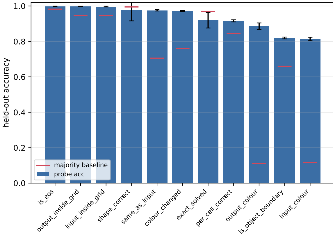
ARC linear-probe decodability (z_H, step 15)
