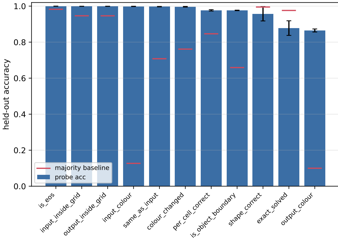
ARC linear-probe decodability (z_L, step 15)
