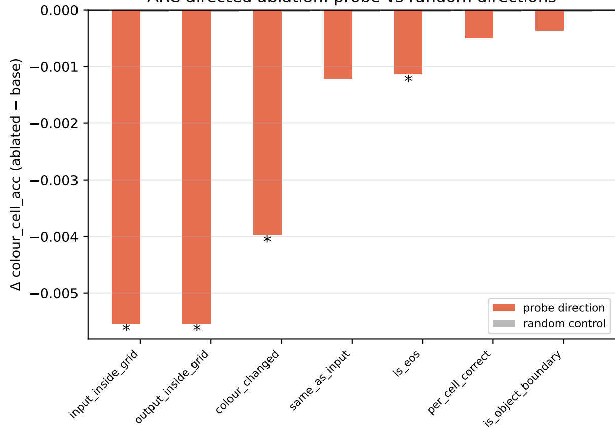
ARC directed ablation: probe vs random directions
