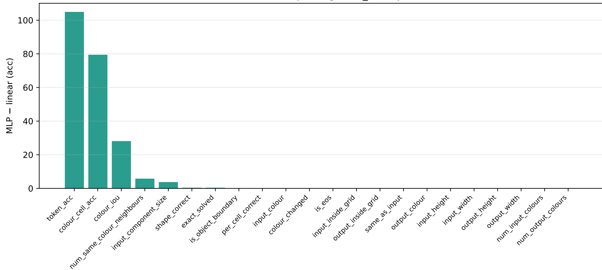
ARC non-linear probe gain (z_H, step 15)
