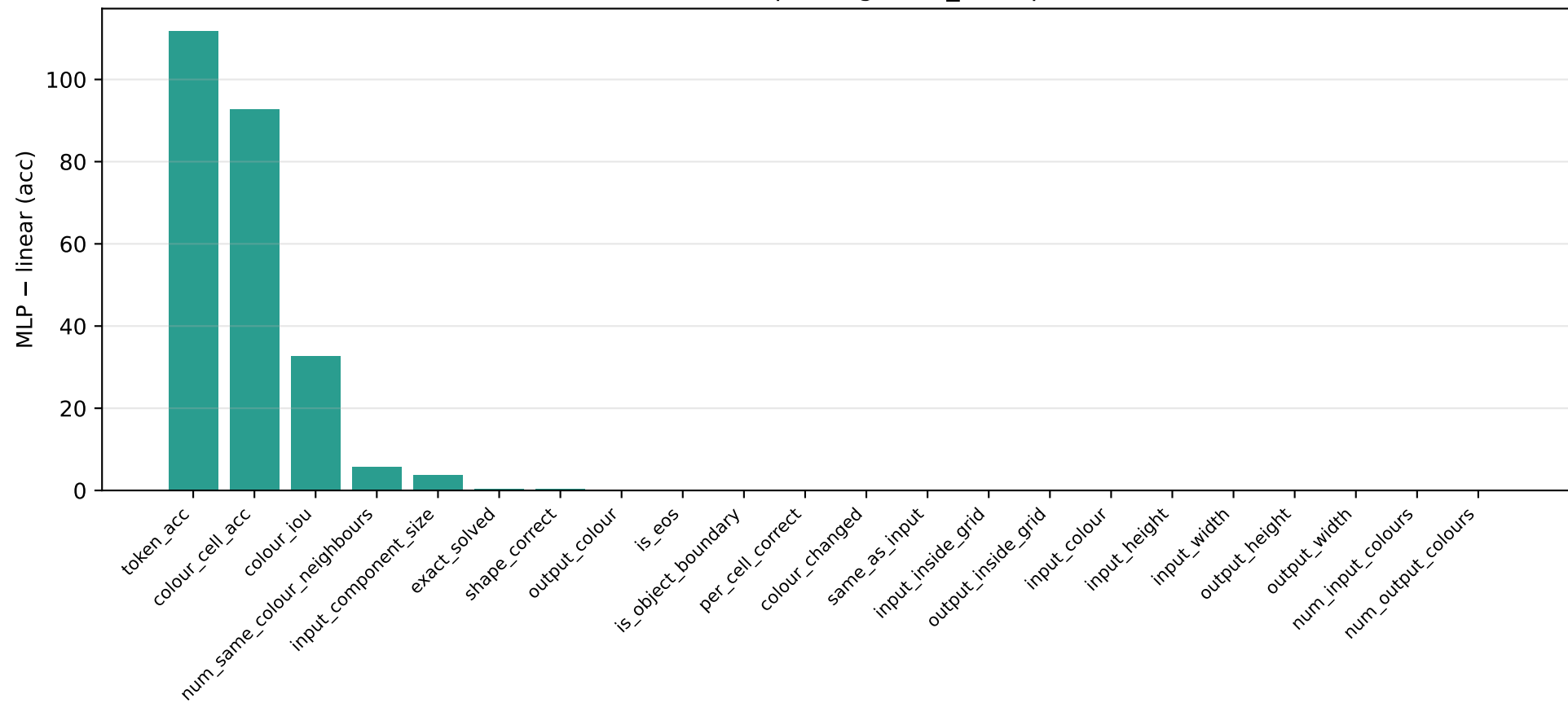
ARC non-linear probe gain (z_L, step 15)
