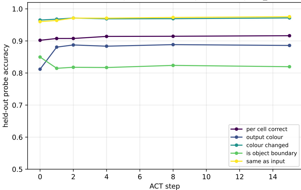
ARC-AGI-2 linear-probe decodability across steps (z_H)
