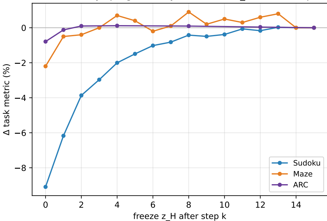
Finding 1: task-dependent refinement depth Sudoku decays progressively; Maze/ARC z_H is a static plan
