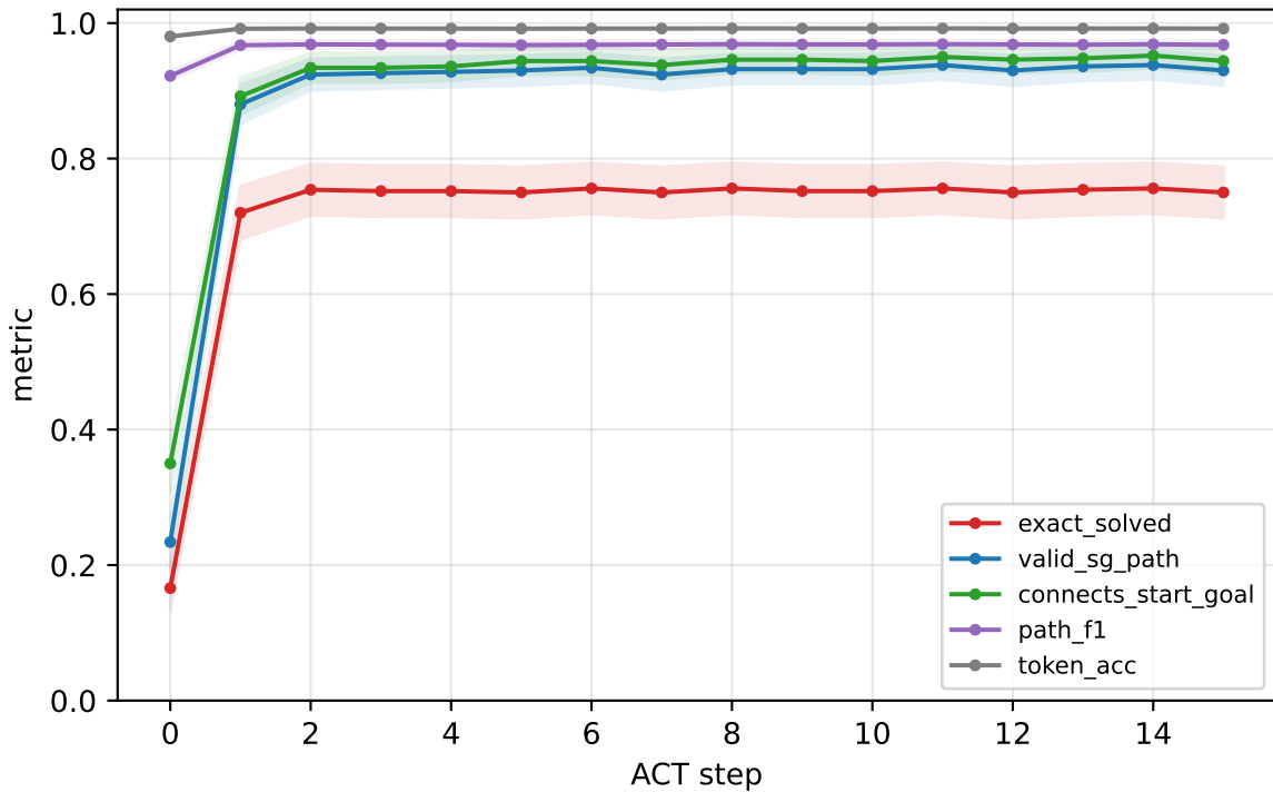
Maze — solution dynamics across ACT steps (N=500)
