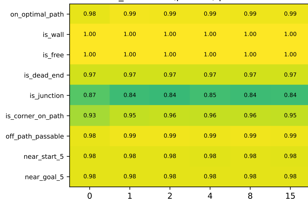
z_H — global (per-puzzle) probe acc
