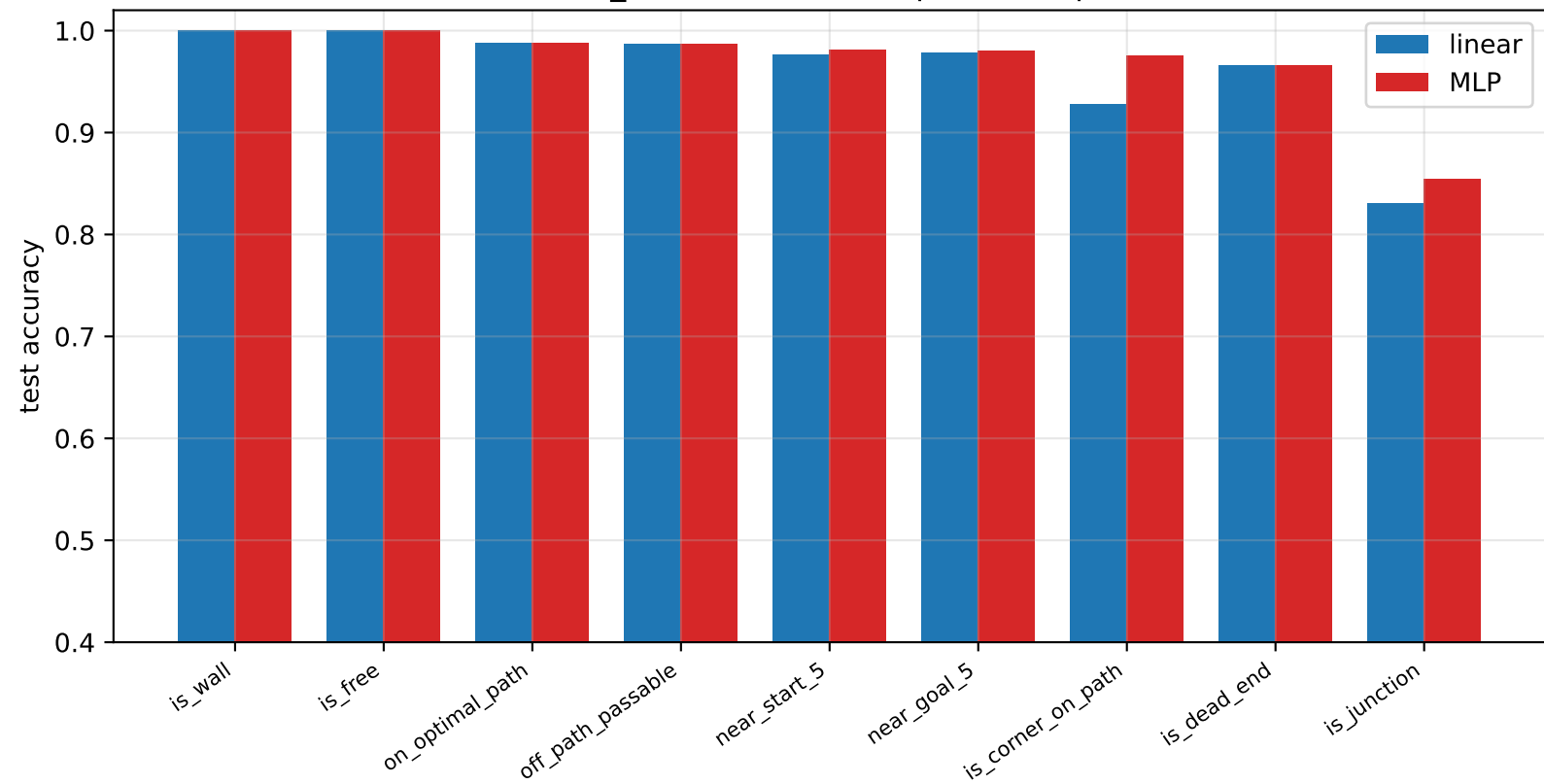
Maze z_H — linear vs MLP probe (step 15)
