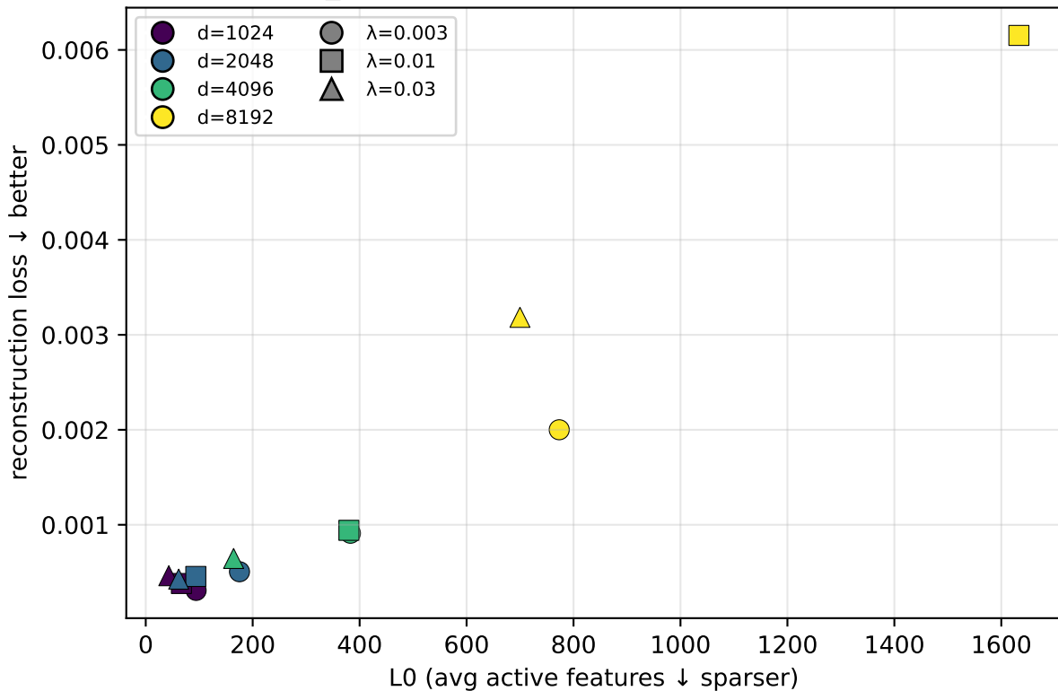
Maze z_H SAE — reconstruction vs sparsity frontier
