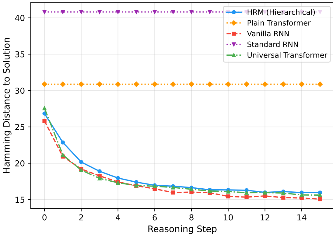
Hamming Distance Convergence
