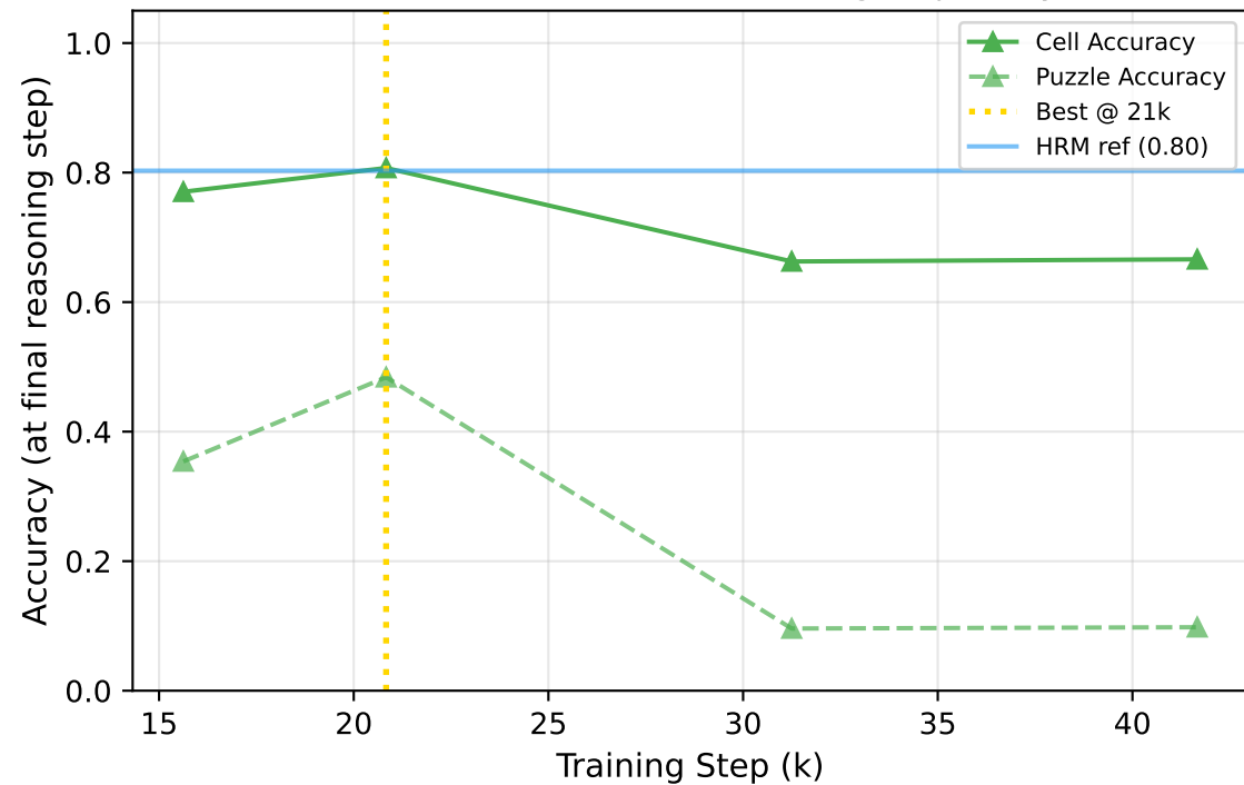
Universal Transformer: Training Trajectory
