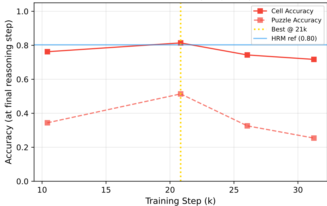
Vanilla RNN: Training Trajectory
