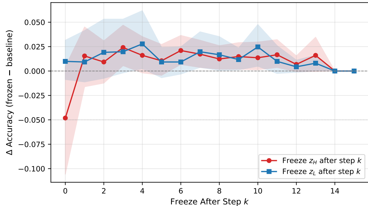
Freeze Crossover: z_H vs z_L
