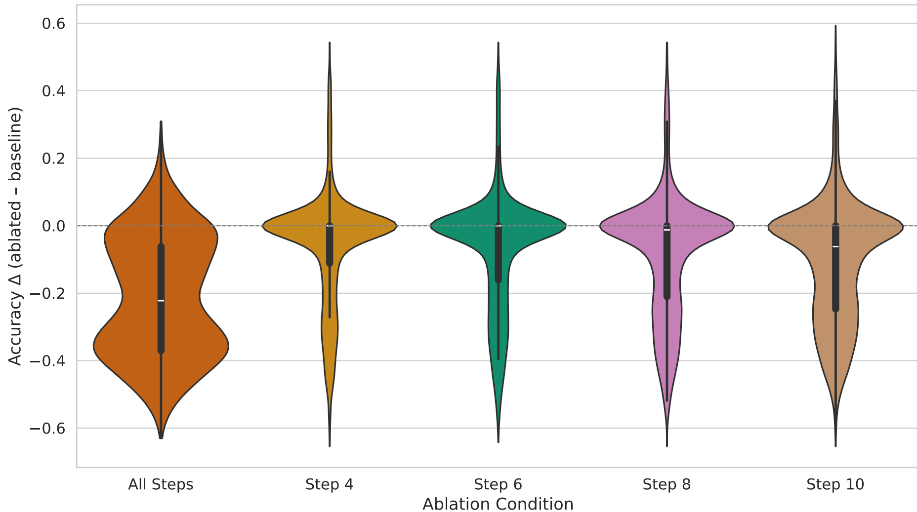
Distribution of Accuracy Changes Under z_H Ablation
