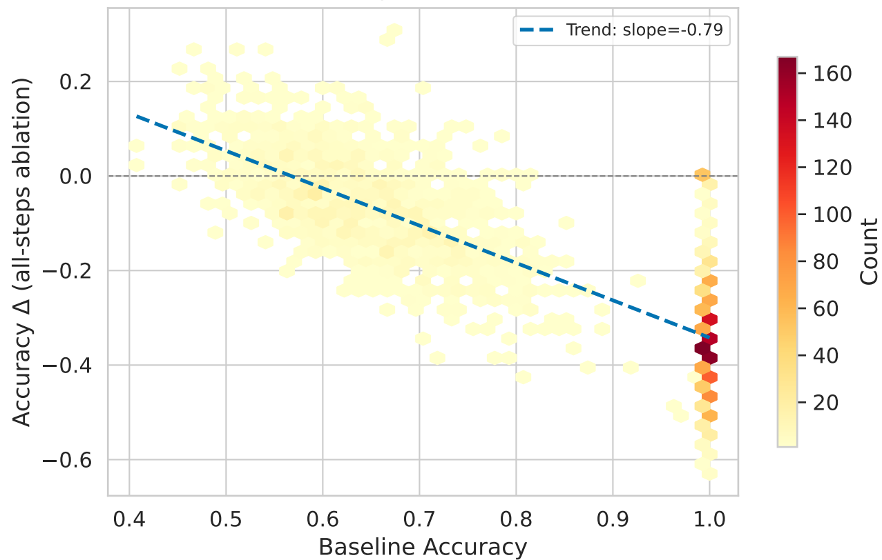
All-Steps z_H Ablation
