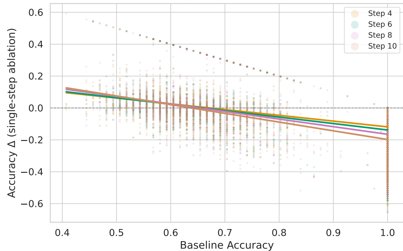
Single-Step z_H Ablation
