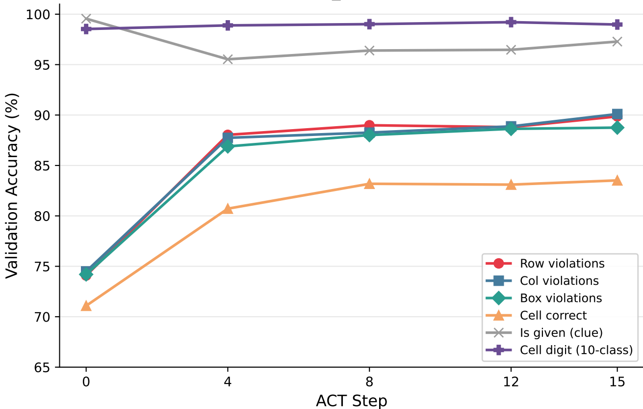
E8: Linear Probe Accuracy by ACT Step (500 puzzles, z_H representations)
