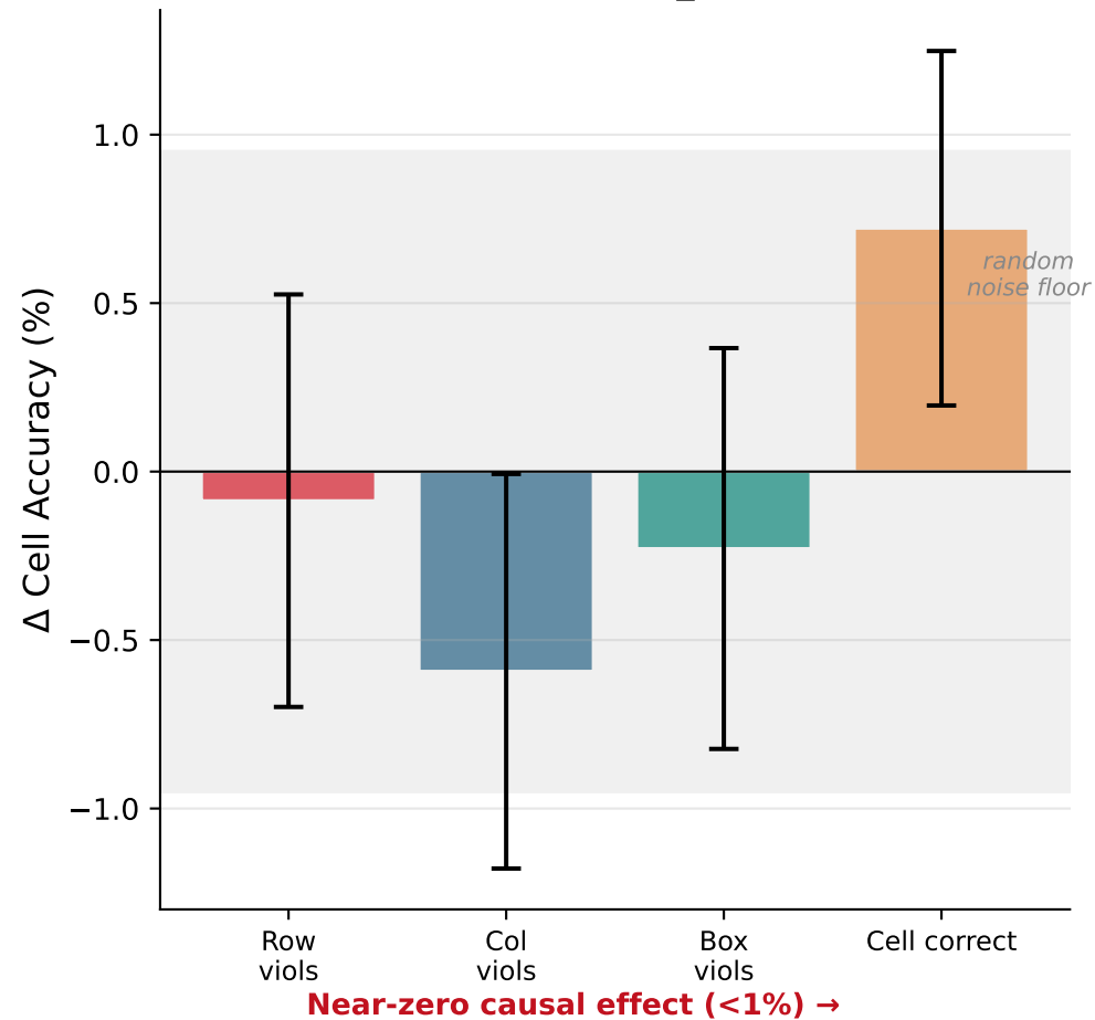
E9: Causal Impact (ablate direction from z_H , 200 puzzles)
