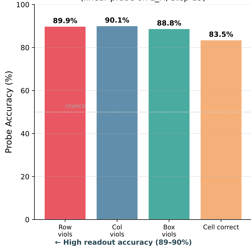
E8: Readout Accuracy (linear probe on z_H , step 15)
