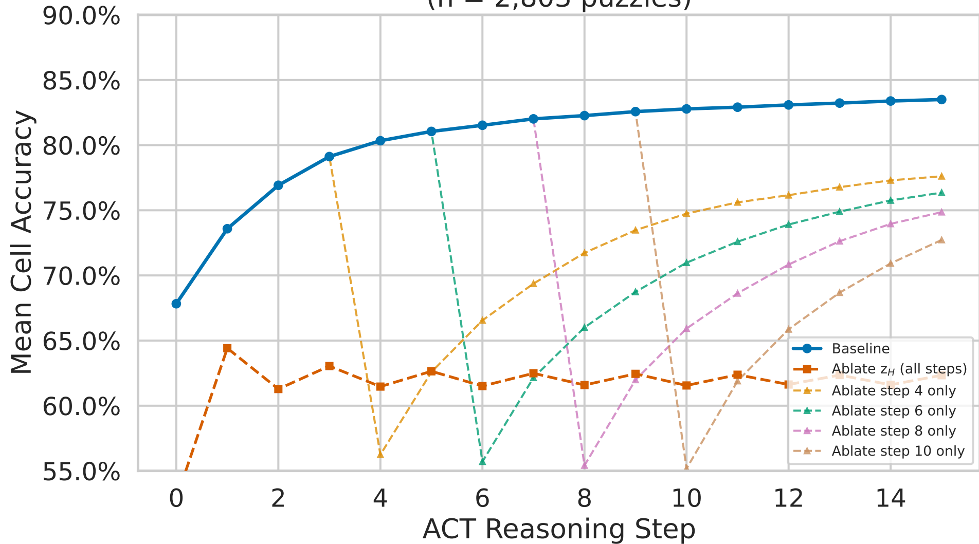
z_H Ablation: Accuracy Across Reasoning Steps (n = 2,803 puzzles)
