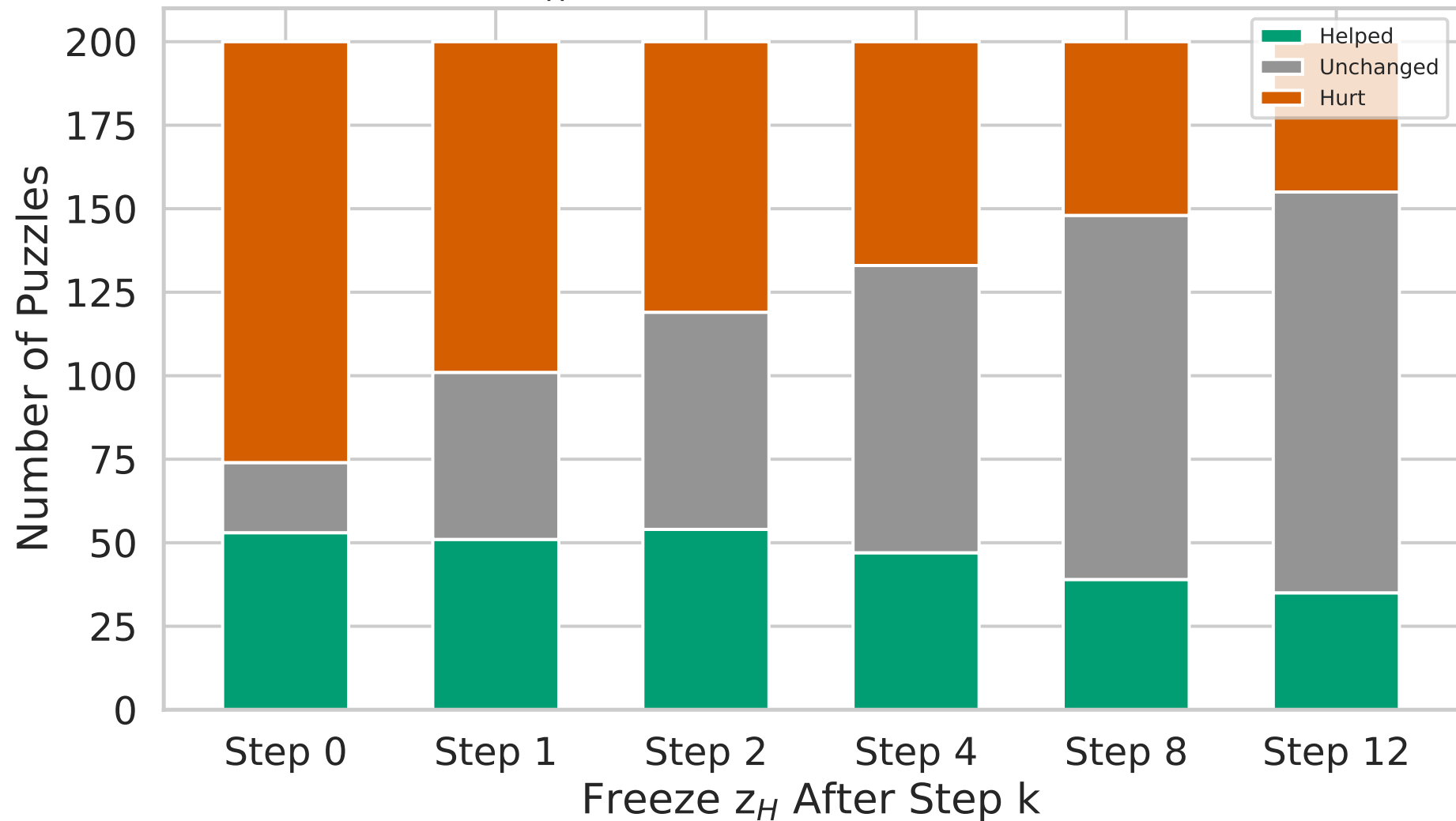
Freeze z_H : Per-Puzzle Outcomes (n = 200)
