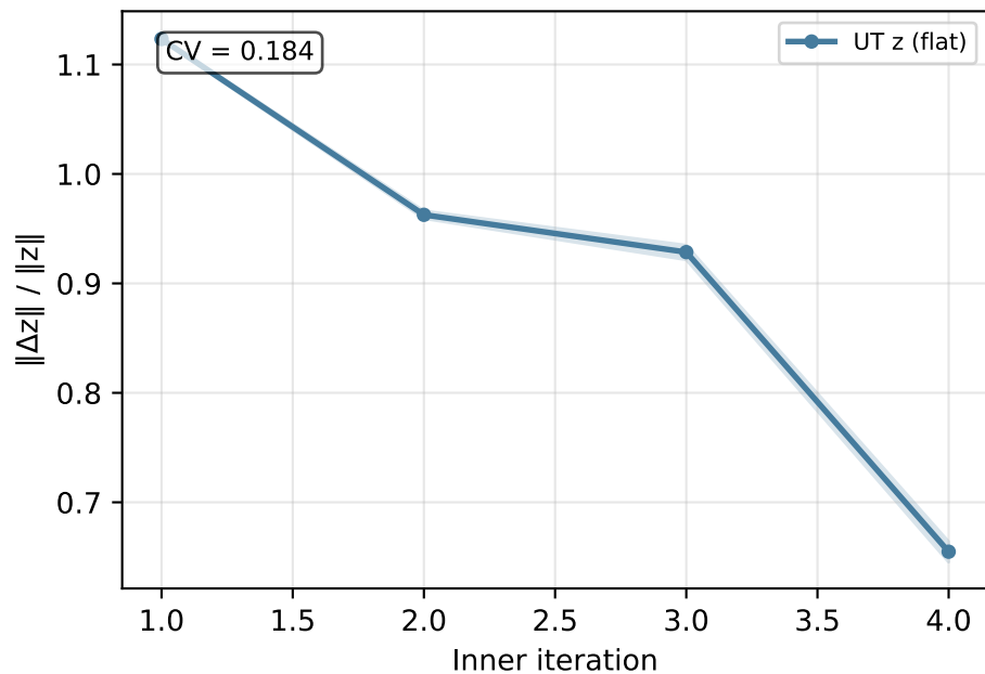
UT: per-iteration change rate (one ACT step)
