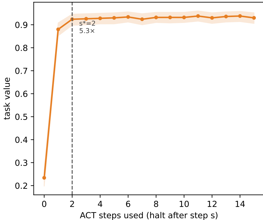
Maze: value vs compute ( \tau=0.01 )
