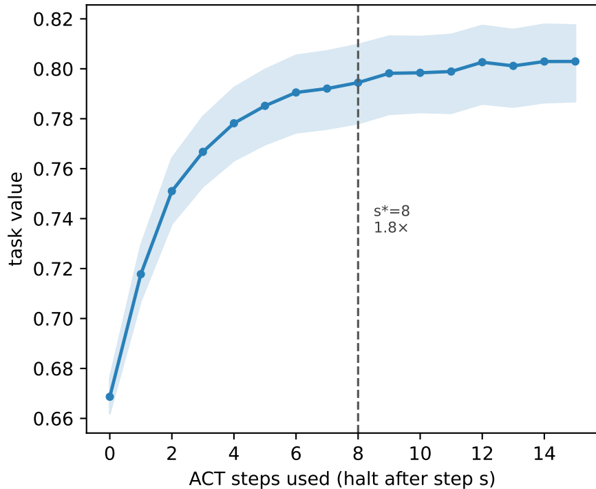
Sudoku: value vs compute ( \tau=0.01 )
