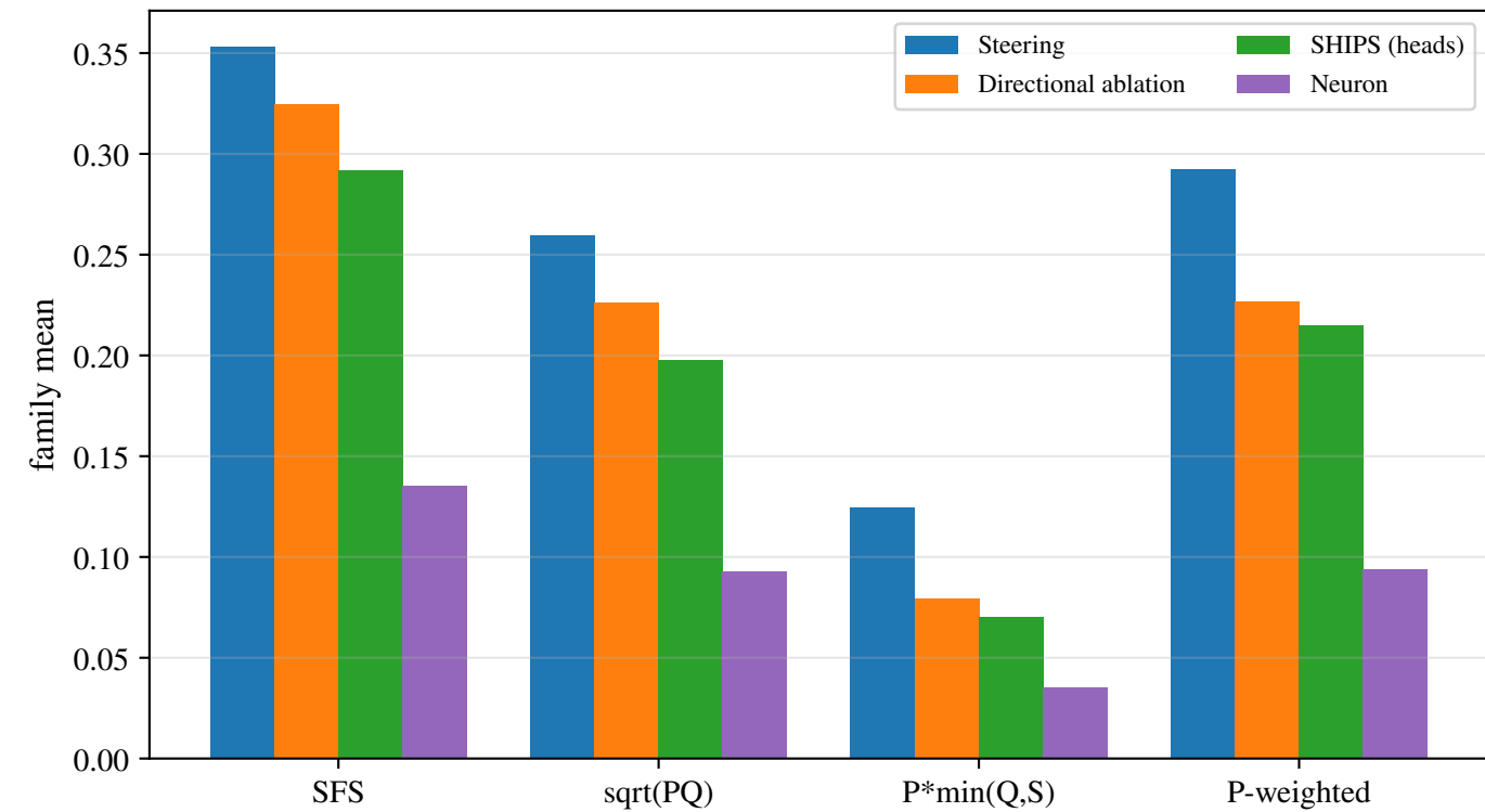
Conclusion is robust to reasonable scalar variants
