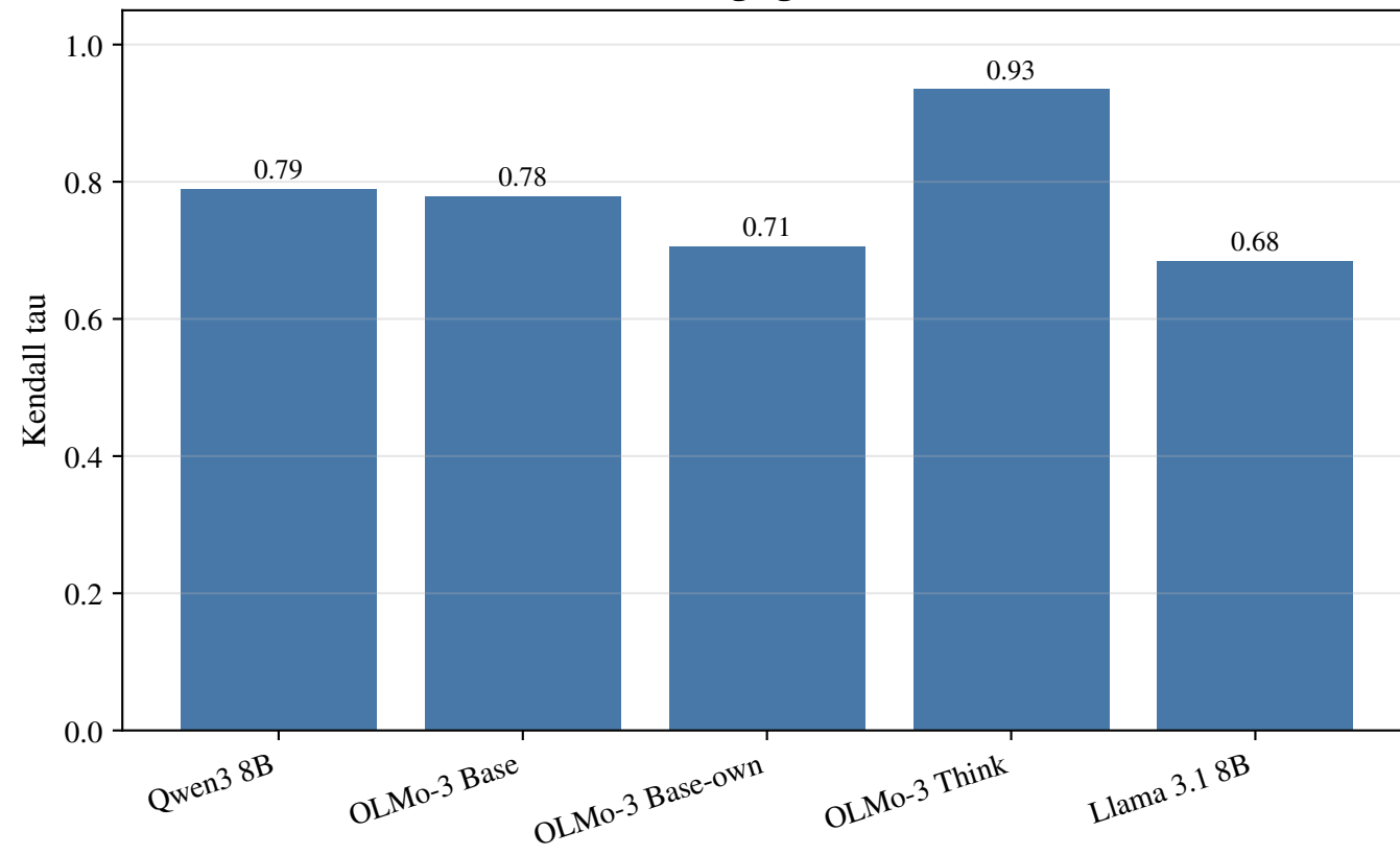
Raw-ASR ranking agreement with SFS
