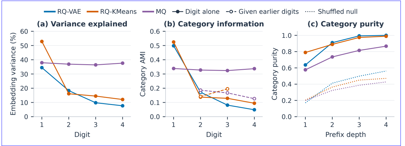
Figure 9: What each digit encodes in the three Industrial 4 \times 128 maps. (a) Item-embedding variance explained by one digit alone. (b) Level-1 category AMI of one digit alone (filled) and given the earlier digits (hollow; shown only where the within-parent estimate is supported). (c) Majority-category purity of multi-item prefix groups (solid) against a shuffled-label null (dotted). At depth four only 0.8% of RQ-VAE items still share a group.
