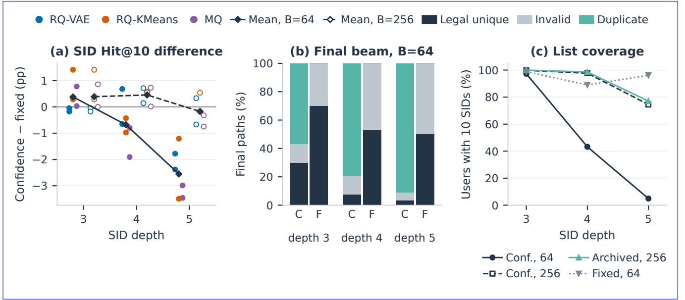
Figure 7: Controlled re-decoding of 18 retained Industrial next-item Diff checkpoints, 6,297 users each. (a) Confidence minus the fixed seed-42 order in SID Hit@10 per checkpoint (filled: B = 64 ; hollow: B = 256 ), with depth means. (b) Final beam at B = 64 : distinct legal SIDs, SIDs absent from the catalog, and duplicate paths to a SID already held; C: confidence, F: fixed. (c) Users who receive ten distinct legal SIDs. “Archived” is the historical decoder, which our search reproduces exactly. Results are conditional on confidence-selected checkpoints and exclude training-seed variation.
