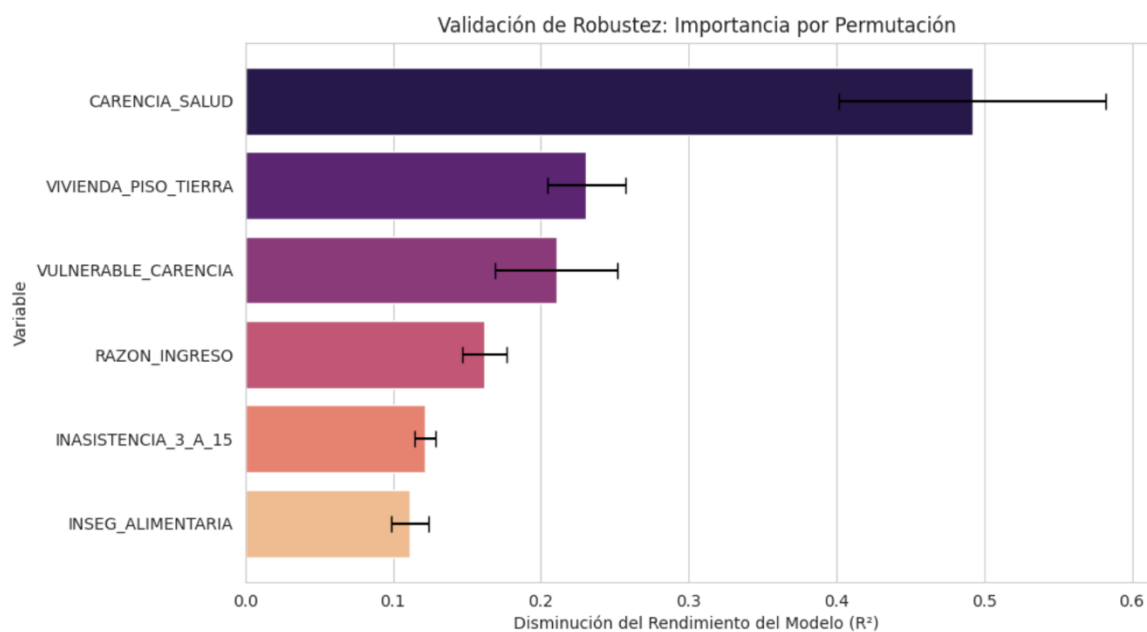
Figura 6 - Permutation Importance
