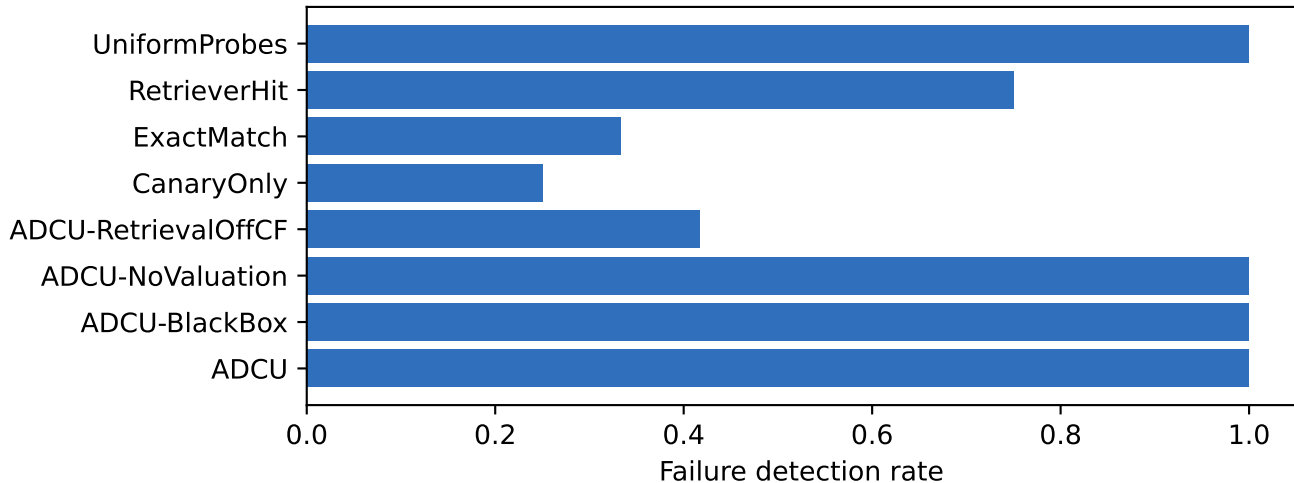
HybridReal detection by audit method
