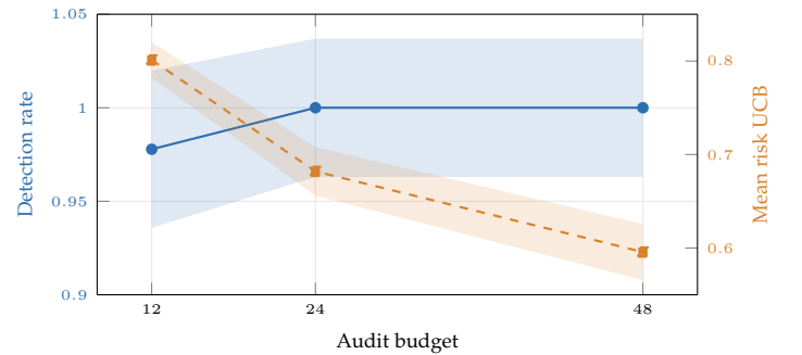
Fig. 7. Audit-budget tradeoff (Table 10). A larger probe budget raises detection (blue, left axis) and lowers the mean risk UCB (orange dashed, right axis) as the Hoeffding confidence floor shrinks.
