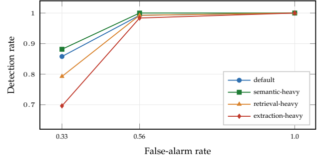
Fig. 3. Detection vs. false alarm across weight profiles as the operating tolerance is swept (Table 14). Lowering the tolerance raises sensitivity, but near the Hoeffding confidence floor it also rejects clean systems; the headline rows instead use the floor-normalized excess-risk tolerance.
