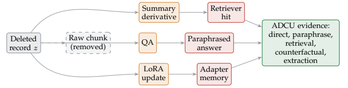
Fig. 4. Case-study provenance graph. The raw chunk of z is syntactically removed (dashed gray), but residual derivatives (orange) keep producing post-deletion behavioral leakage (red) that ADCU catches through its evidence channels (green)—the orphan-derivative term \gamma_z in the composition theorem.
