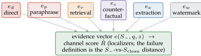
Fig. 5. The six diagnostic evidence channels referenced in Section 4. Each fires under a different failure mode—direct/paraphrase under model-side leakage, retrieval under stale or shadow-copy artifacts, counterfactual under any S_- -vs- S_{\text{clean}} divergence, extraction under adversarial probes, watermark under canary or provenance-token hits—and together they localize residual dependence without themselves defining deletion failure.
