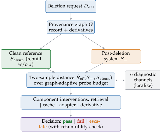
Fig. 2. ADCU audit pipeline. A deletion request is expanded through the provenance graph; the post-deletion system S_- is compared against the clean reference S_{clean} via a two-sample distance over a graph-adaptive probe budget, six diagnostic channels localize where any residual dependence is mediated, component interventions attribute it causally, and the audit returns a confidence-bounded decision with a retain-utility check.
