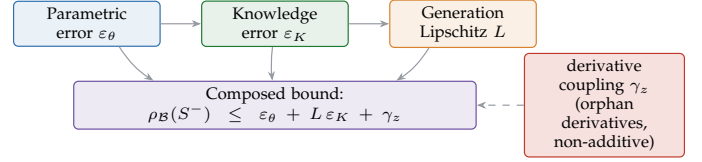
Fig. 1. Pipeline-deletion composition (Appendix A). Per-component deletion errors compose additively— \varepsilon_\theta on parameters, \varepsilon_K on knowledge amplified by the generation Lipschitz factor L —plus a non-additive derivative-coupling term \gamma_z that is zero iff every derivative of the deleted record has also been removed; otherwise orphan derivatives dominate.
