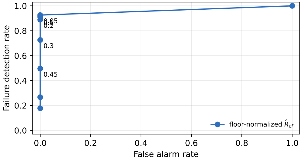
Counterfactual ROC after floor normalization
