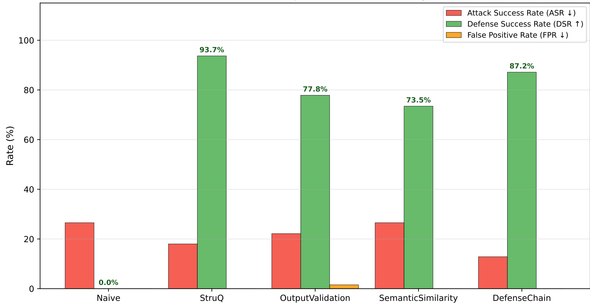
BidPoison: Defense Comparison Across 5 Configurations
