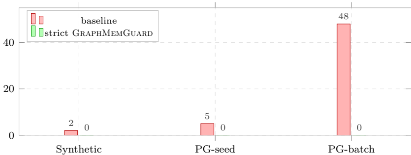
Leaked victim-owned edges
