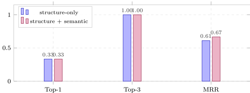
Accuracy / MRR
