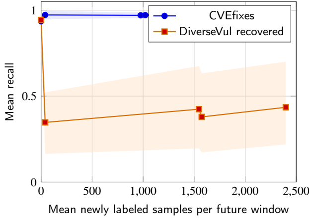
Figure 3: Policy-vs-label-cost view under unseen-project temporal testing.
