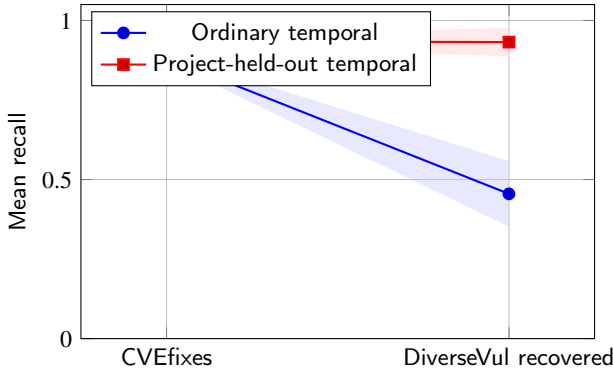
Figure 4: Ordinary temporal versus project-held-out no-refresh evaluation.
