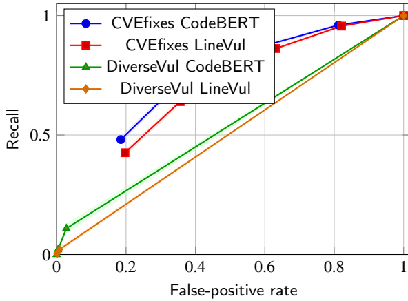
Figure 6: Threshold/FPR tradeoff for project-held-out neural runs.
