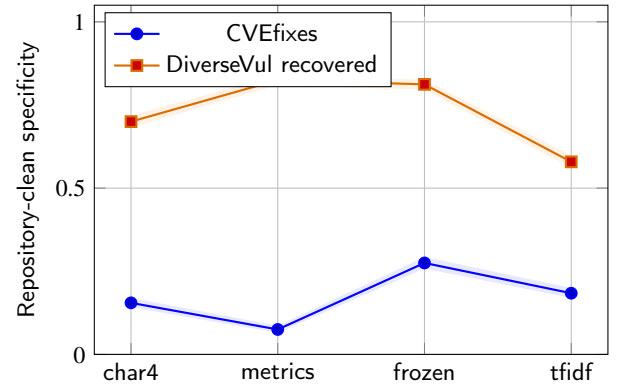
Figure 7: Repository-clean specificity benchmark.
