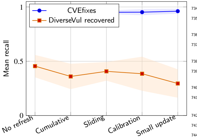
Figure 8: Maintenance-policy mean recall with bootstrap uncertainty.
