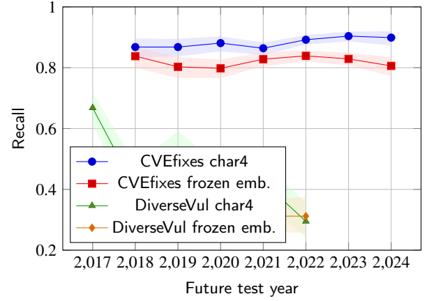
Figure 5: Fixed-origin future recall curves with uncertainty bands.
