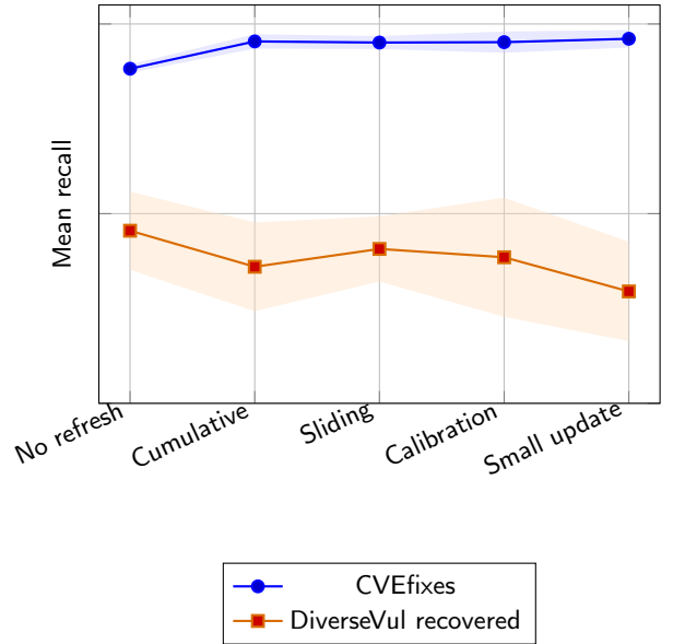
Figure 8: Maintenance-policy mean recall with bootstrap uncertainty.
