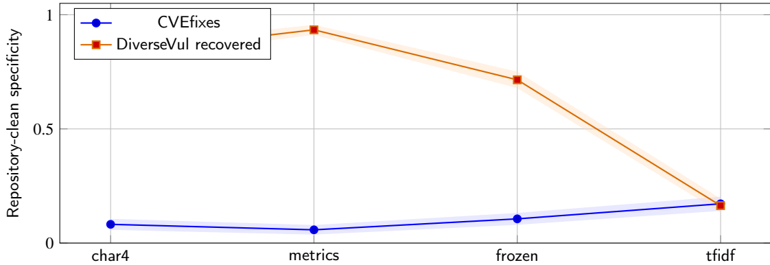
Figure 7: Repository-clean specificity benchmark. Lines show specificity by detector family and shaded bands are Wilson 95% intervals computed from true-negative and false-positive counts on the 634 clean-only functions.
