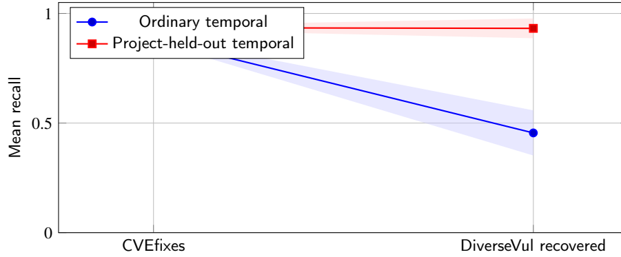
Figure 4: Ordinary temporal versus project-held-out no-refresh evaluation for the primary character baseline. Higher project-held-out recall does not mean the examples are easier; it is coupled to a different threshold/FPR regime and very high false-positive rates, so it must be reported separately from ordinary chronological evaluation. Error bars are 95% intervals.
