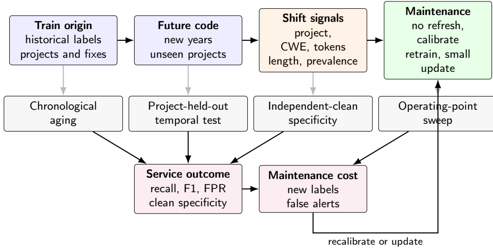
Figure 1: Visual summary of detector maintenance in MAINT-VD. A detector is evaluated as a maintained artifact: historical labels define a train origin, future years and unseen projects induce shift, maintenance policies and threshold rules choose an operating point, and the result is judged by service outcomes and costs.
