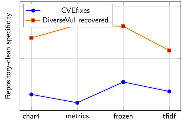
Figure 7: Repository-clean specificity benchmark.
