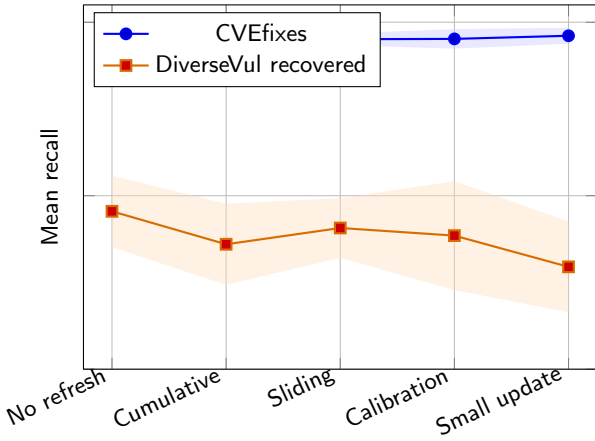
Figure 8: Maintenance-policy mean recall with bootstrap uncertainty.
