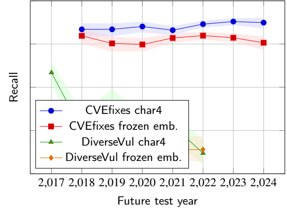
Figure 5: Fixed-origin future recall curves with uncertainty bands.
