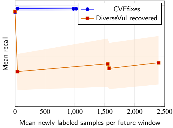
Figure 3: Policy-vs-label-cost view under unseen-project temporal testing.
