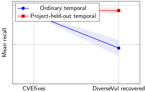
Figure 4: Ordinary temporal versus project-held-out no-refresh evaluation.
