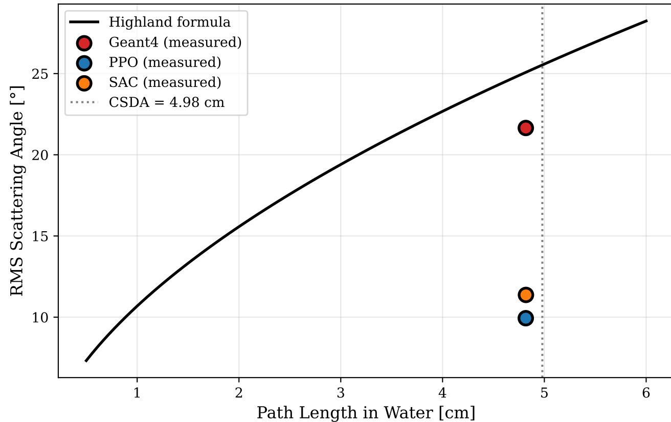
Highland Formula vs Measured Scattering
