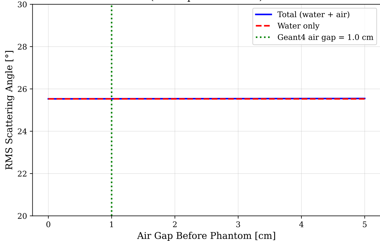
Effect of Air Gap on Scattering (Water path = 5.0 cm)
