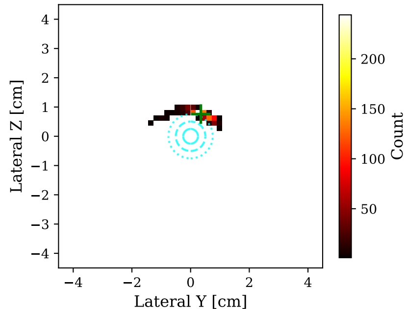
SAC Cross-Section View \sigma = 0.25 \text{ cm} Bias: (+0.35, +0.76)
