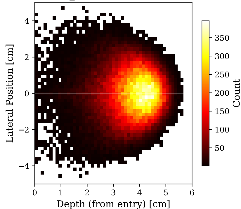
Geant4 (Reference) Side View (like density texture) \sigma_{\text{lateral}} = 1.20 \text{ cm}
