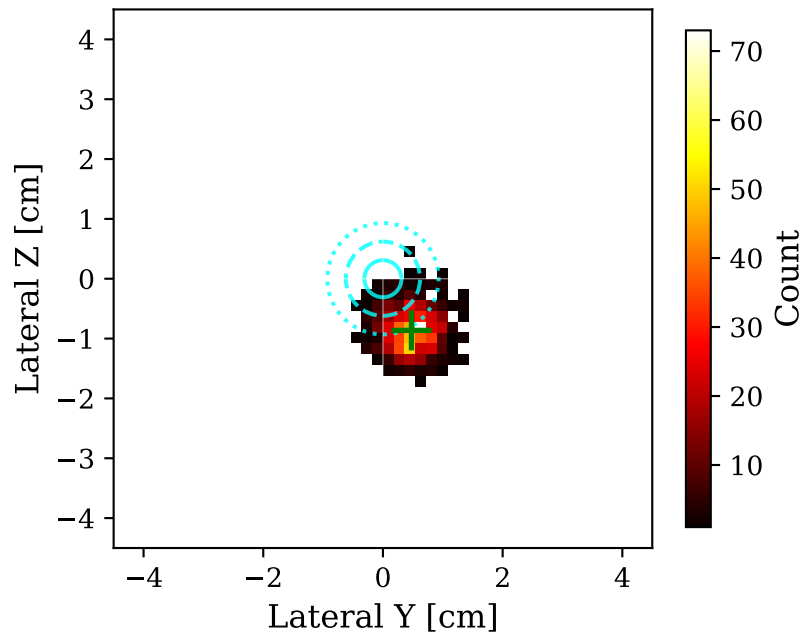
PPO Cross-Section View \sigma = 0.31 \text{ cm} Bias: (+0.48, -0.86)
