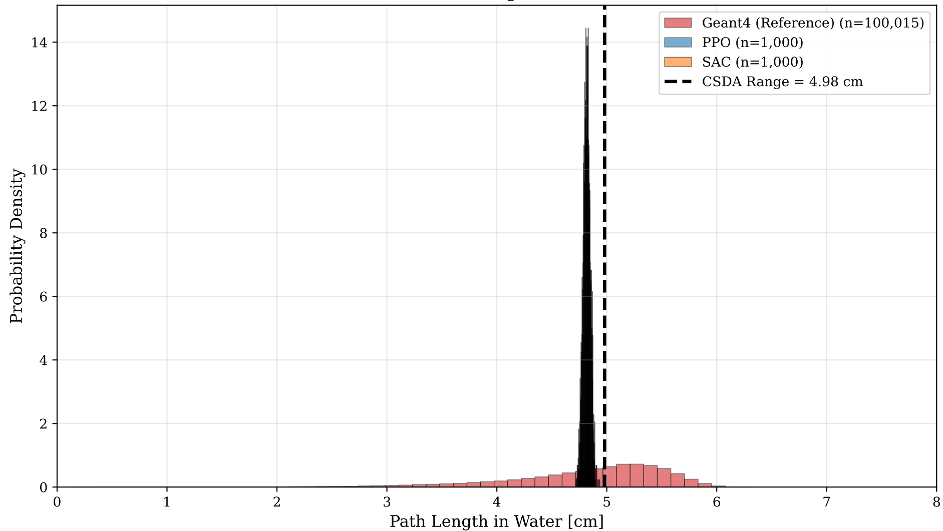
Electron Path Length Distribution
