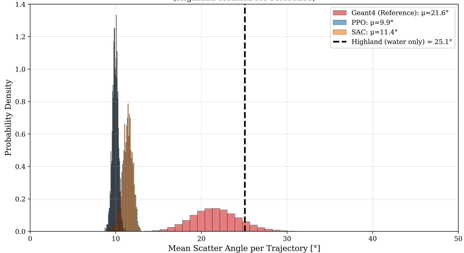
Scattering Angle Distribution (Highland formula for reference)
