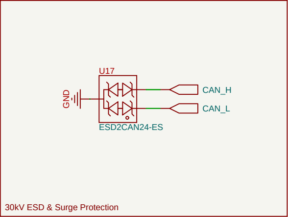
30kV ESD & Surge Protection
