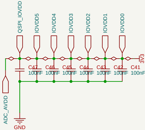
3V3 Decoupling Capacitors
