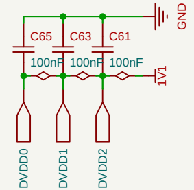
1V1 Decoupling Capacitors
