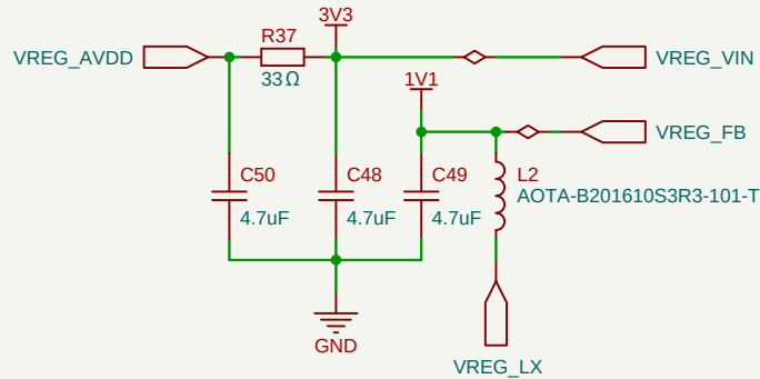
External Core Regulator Components
