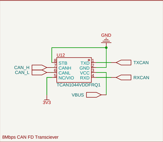
8Mbps CAN FD Transceiver
