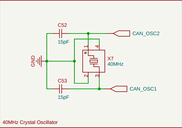
40MHz Crystal Oscillator
