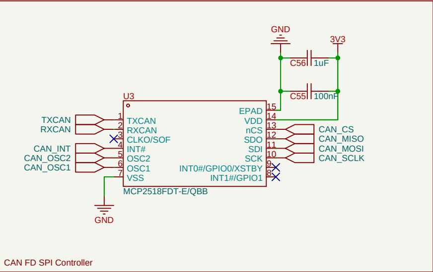
CAN FD SPI Controller
