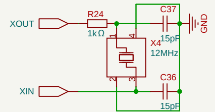
12MHz Crystal Oscillator
