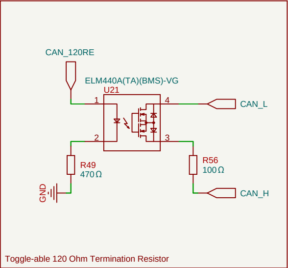
Toggle-able 120 Ohm Termination Resistor
