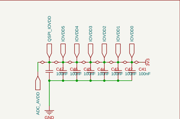
3V3 Decoupling Capacitors
