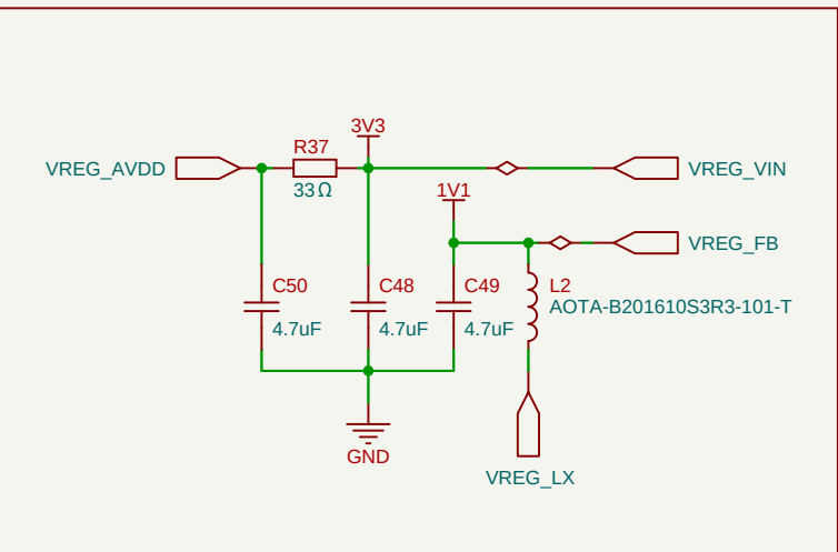
External Core Regulator Components
