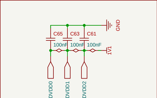
1V1 Decoupling Capacitors
