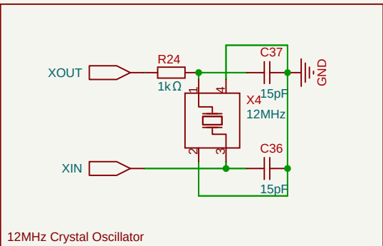
12MHz Crystal Oscillator
