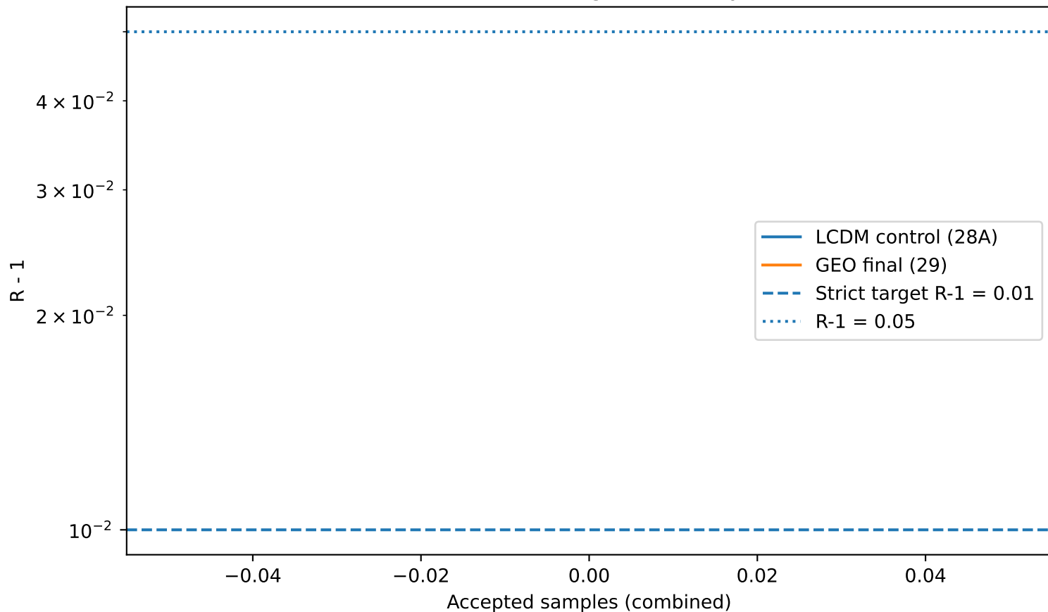
MCMC convergence history
