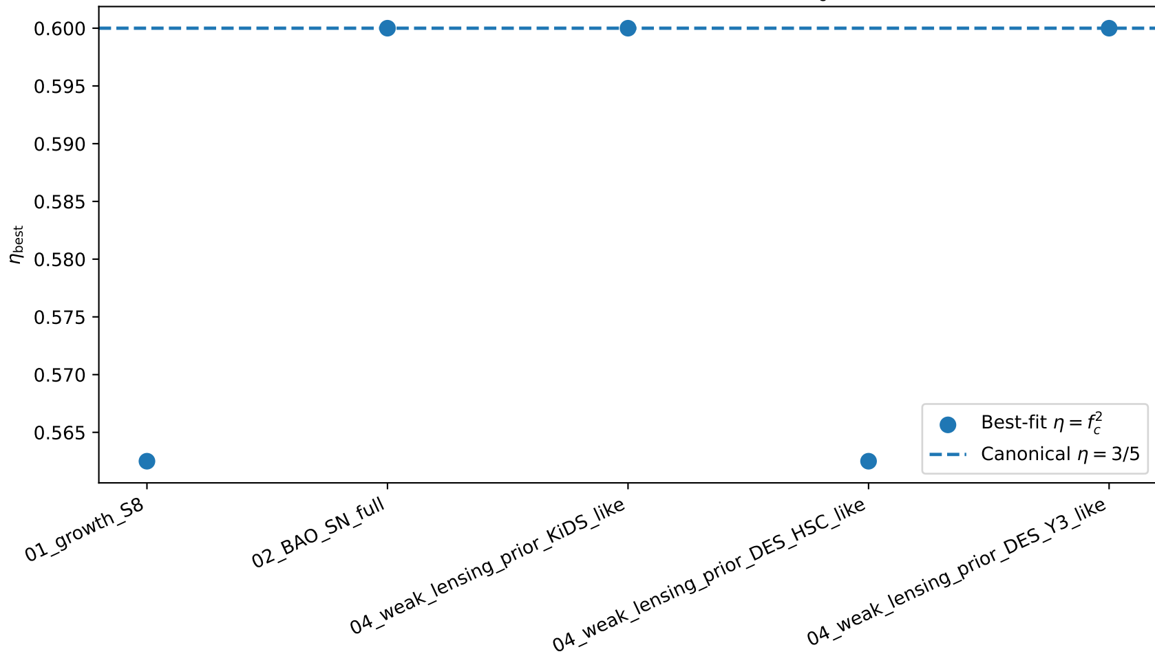
Cross-configuration stability of \eta = f_c^2
