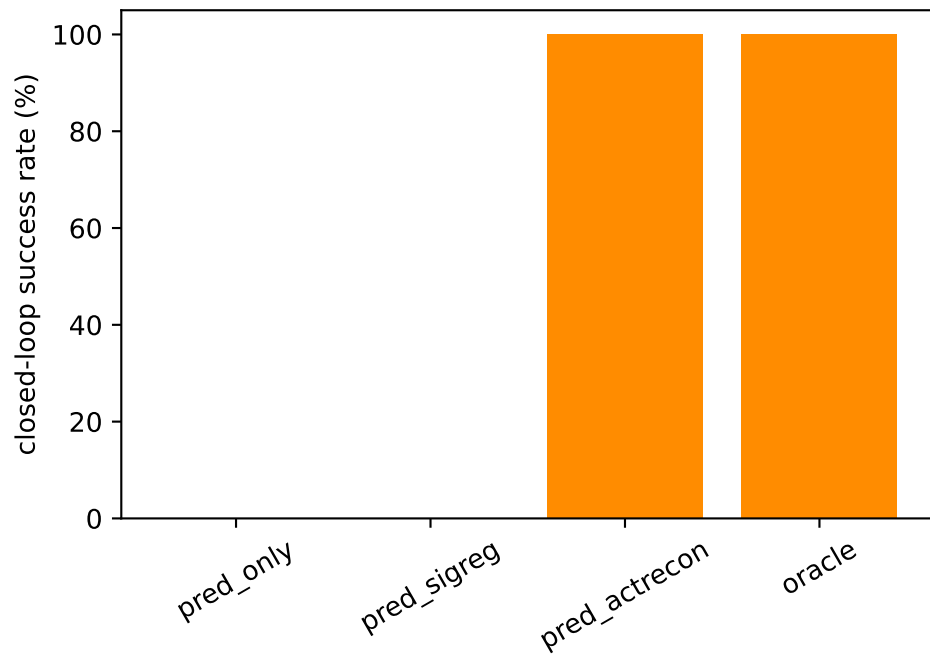
Representation collapse vs closed-loop controllability
